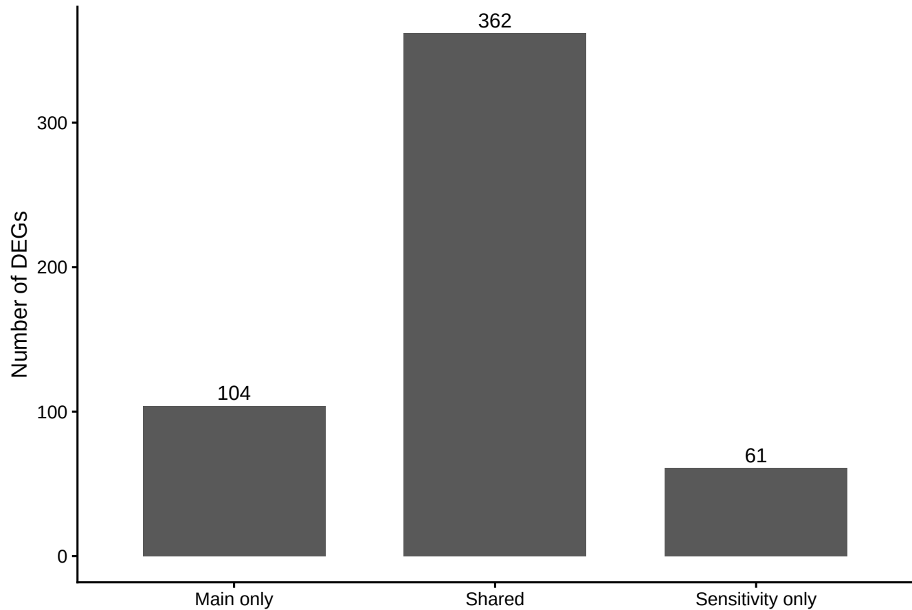
DEG overlap between models
